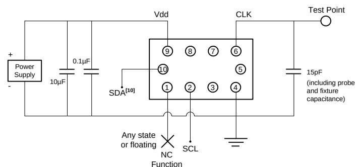
Figure 12. LVCMOS Test Circuit ( I^2C Control), DCTCXO mode
