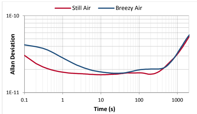
Figure 19. ADEV
