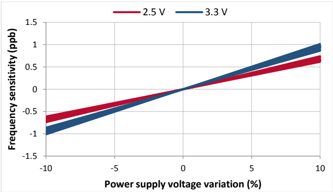
Figure 28. VDD sensitivity
