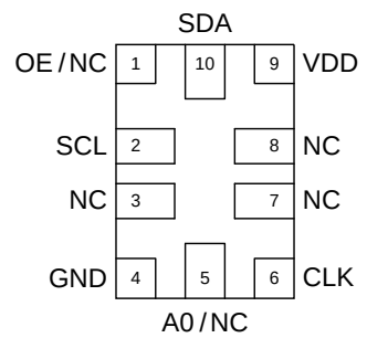
Figure 5. DCTCXO
