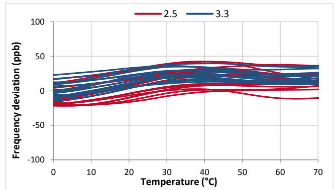
Figure 22. Frequency vs Temperature
