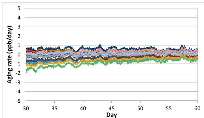
Figure 25. 1-day aging rate (to 62 days)
