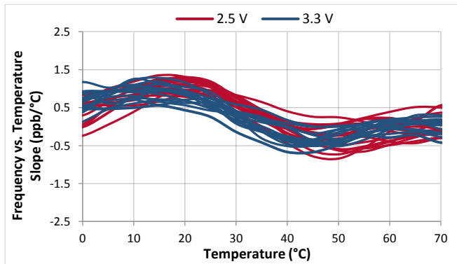
Figure 23. Freq. vs. Temp. Slope ( \Delta f/\Delta T )
