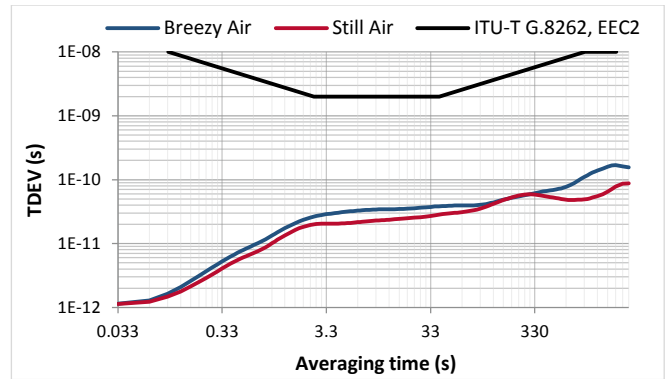
Figure 20. TDEV (0.1 Hz loop bandwidth)
