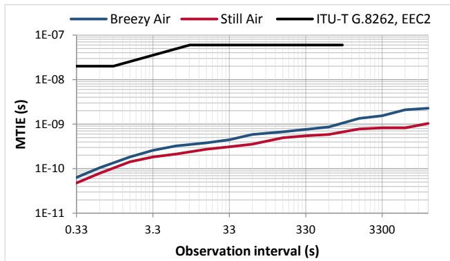
Figure 21. MTIE (0.1 Hz loop bandwidth)
