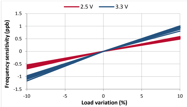
Figure 27. Load sensitivity
